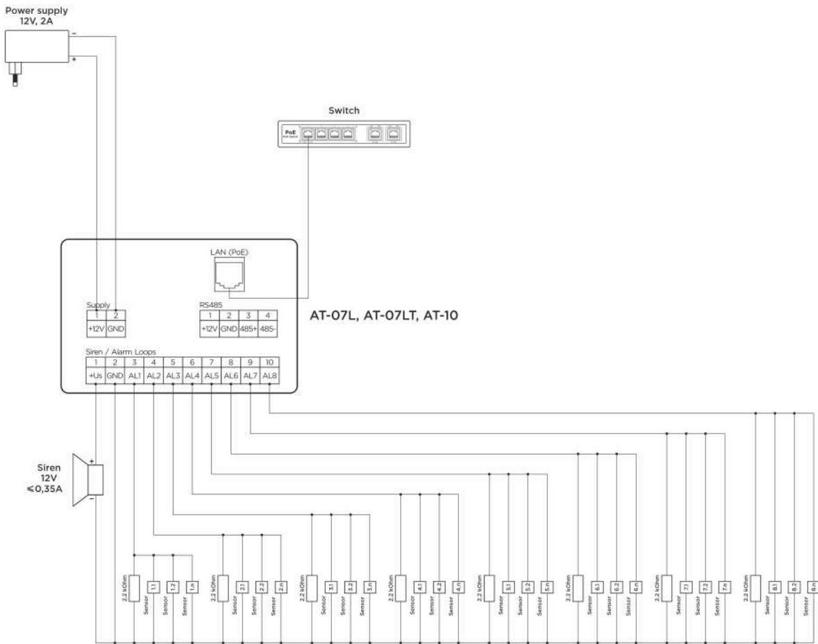
Wiring diagram for security alarm sensors with NO - normally open contact types
